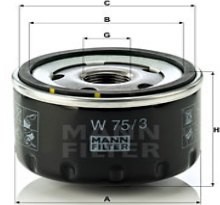
Oil Filter W 75/3 EM-10180
