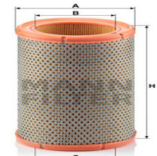
Air Filters C 1380 EM-30360
