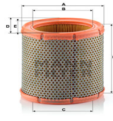
Air Filters C 1460 EM-30347
