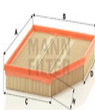
Air Filters C 31 149 EM-30142
